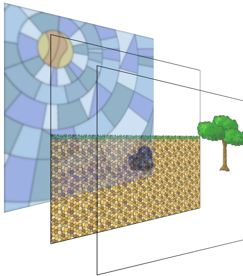
Figure 145: A small example of the “painter’s algorithm”
